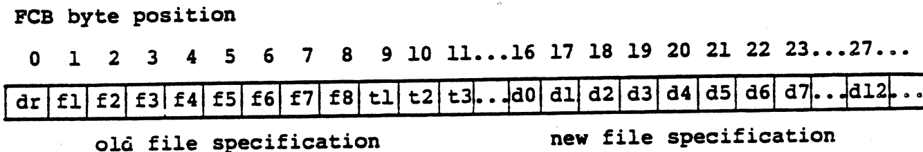
Figure 4-1. FCB Format for Rename Function
