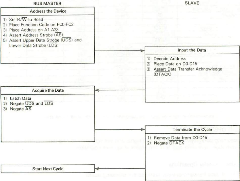
Figure 4-2. Word Read Cycle Flowchart
