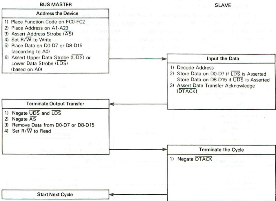
Figure 4-7. Byte Write Cycle Flowchart
