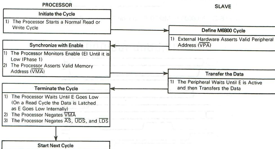
Figure 6-1. M6800 Interfacing Flowchart
