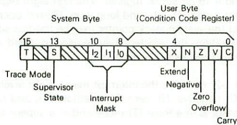
Figure 1-2. Status Register
