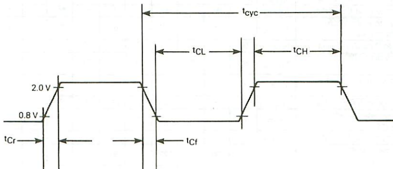
Figure 8-5. Clock Input Timing Diagram
