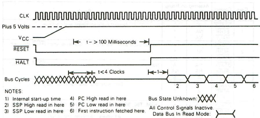
Figure 4-21. Reset Operation Timing Diagram
