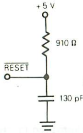
Figure 8-1. \overline{\text{RESET}} Test Load
