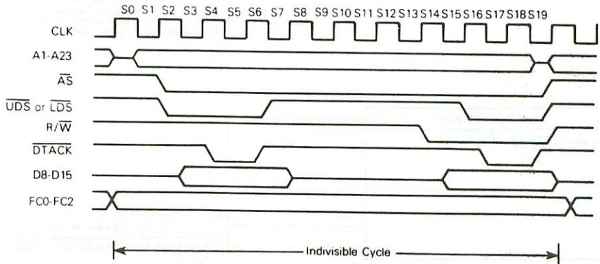
Figure 4-10. Read-Modify-Write Cycle Timing Diagram
