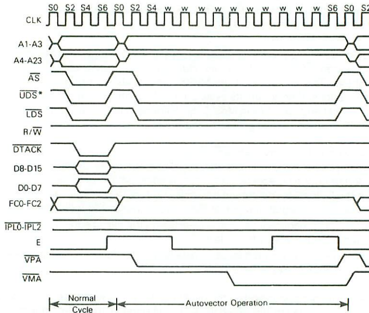
Figure 6-4. Autovector Operation Timing Diagram
