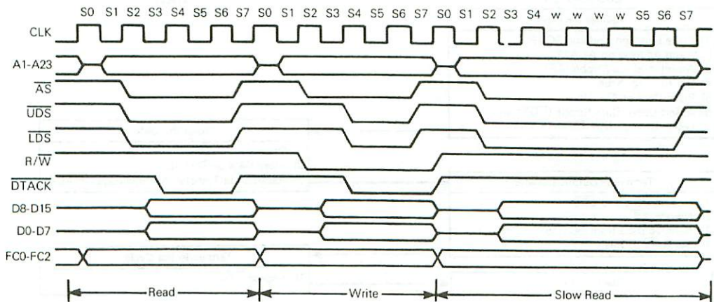
Figure 4-4. Read and Write Cycle Timing Diagram
