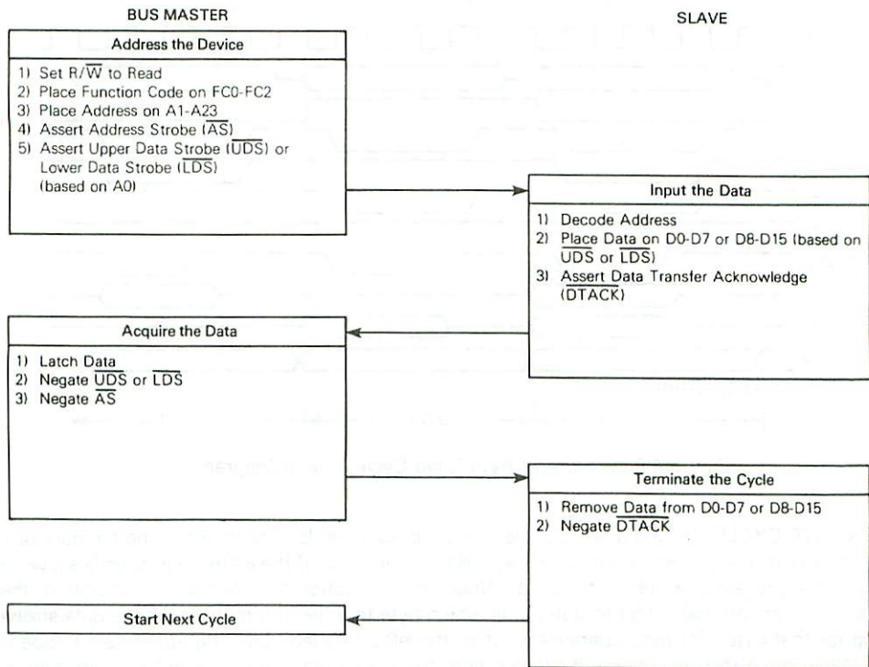
Figure 4-3. Byte Read Cycle Flowchart
