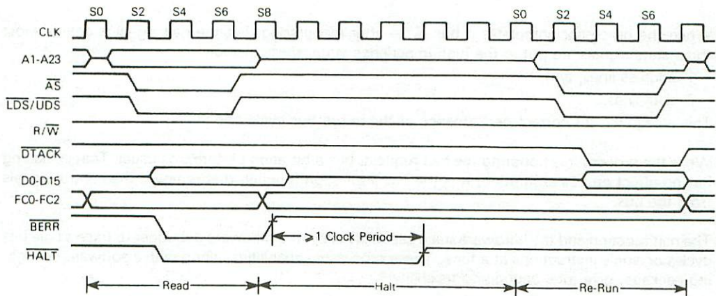
Figure 4-19. Re-Run Bus Cycle Timing Diagram
