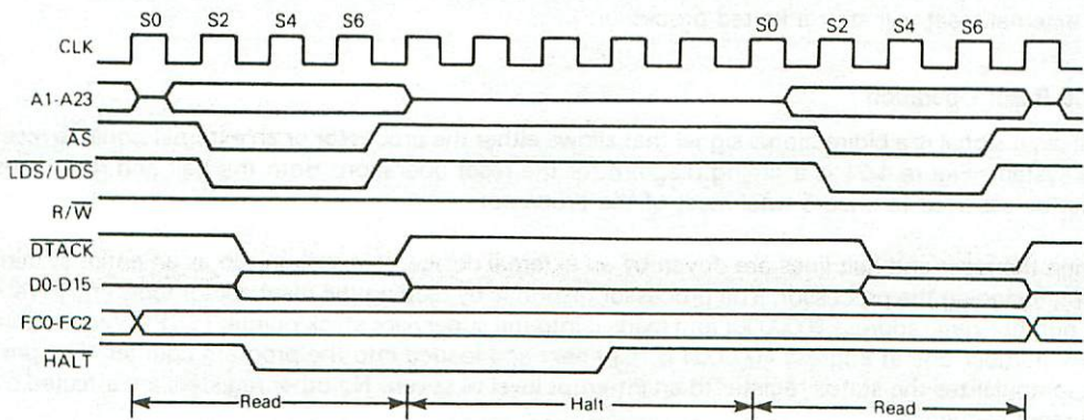
Figure 4-20. Halt Processor Timing Diagram
