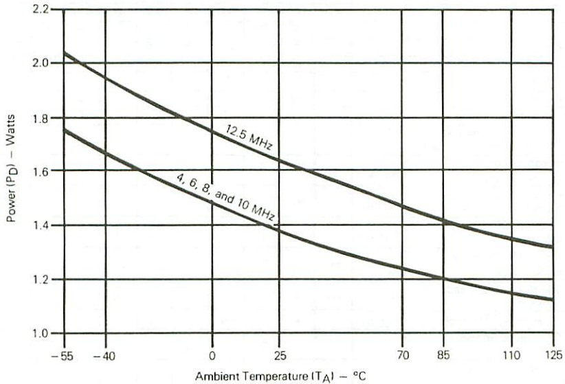
Figure 8-4. MC68000 Power Dissipation ( P_D ) vs Ambient Temperature ( T_A )
