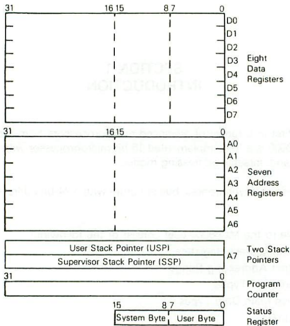
Figure 1-1. Programming Model
