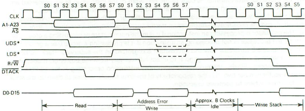
Figure 5-9. Address Error Timing Diagram
