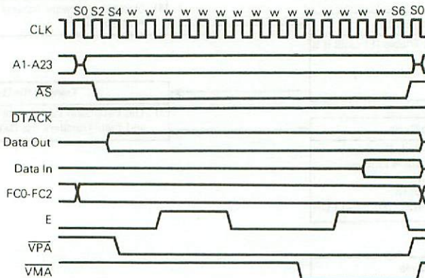
Figure 6-3. MC68000 to M6800 Peripheral Timing — Worst Case
