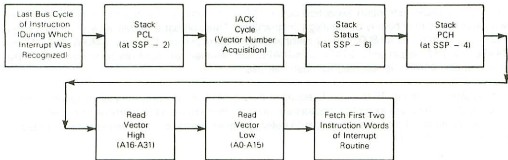
Figure 5-7. Interrupt Processing Sequence
