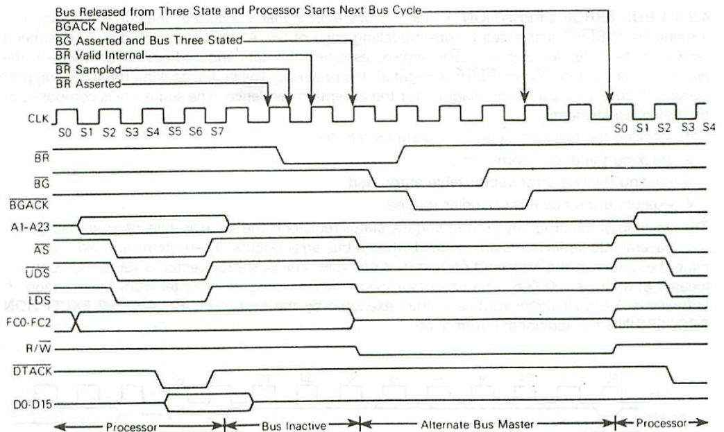
Figure 4-16. Bus Arbitration Timing Diagram – Bus Inactive
