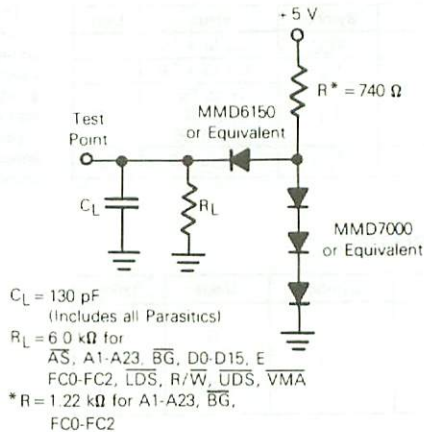
Figure 8-3. Test Loads
