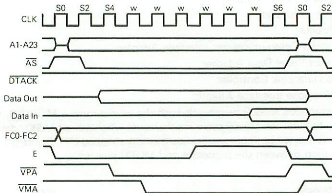
Figure 6-2. MC68000 to M6800 Peripheral Timing — Best Case
