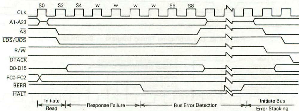
Figure 4-18. Bus Error Timing Diagram
