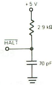
Figure 8-2. \overline{\text{HALT}} Test Load
