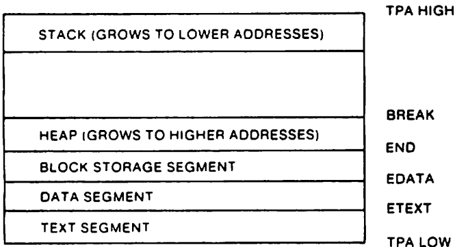
Figure 1-1. Memory Layout
