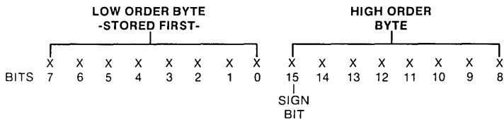
Figure 5-4. Integer Storage
