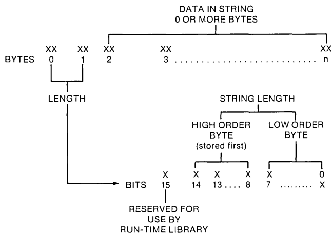
Figure 5-5. String Storage
