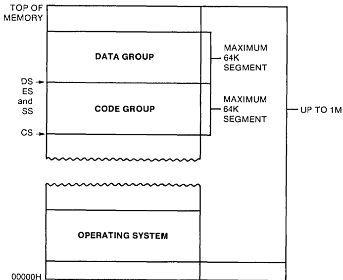
Figure 5-1. Memory Allocation
