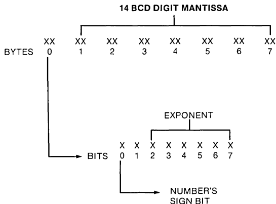
Figure 5-3. Real Number Storage
