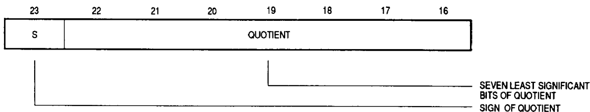
Figure 5. Quotient Byte
