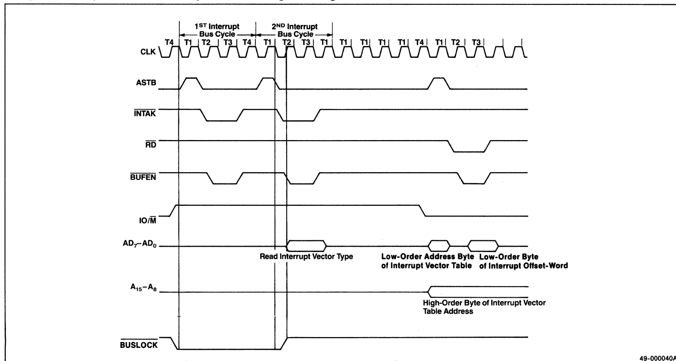
Figure 6-2. μPD70108 Interrupt Acknowledge Timing
