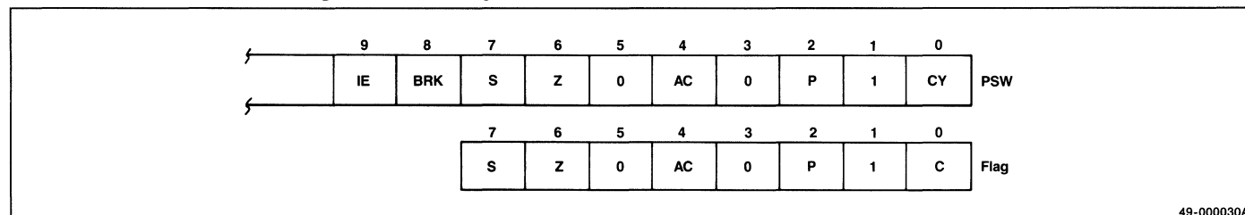
Figure 8.2. Corresponding PSW and Flags
