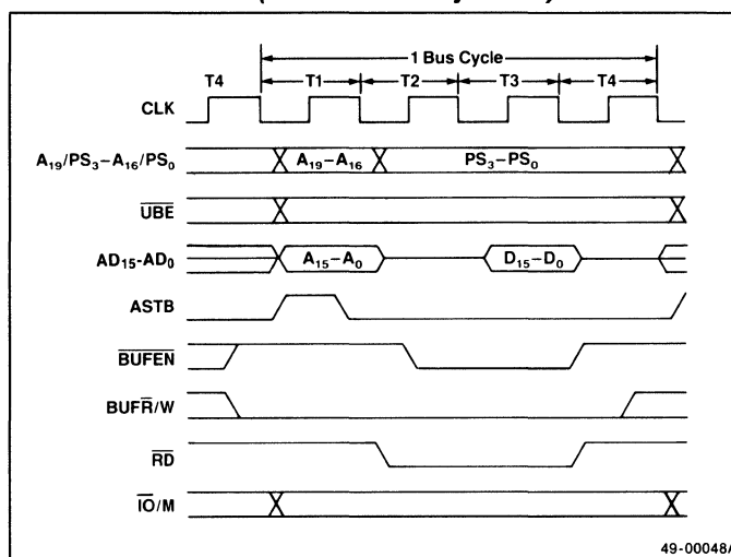
Figure 5-3. Read Timing of \mu PD70116 Memory and I/O (Small-Scale Systems)
