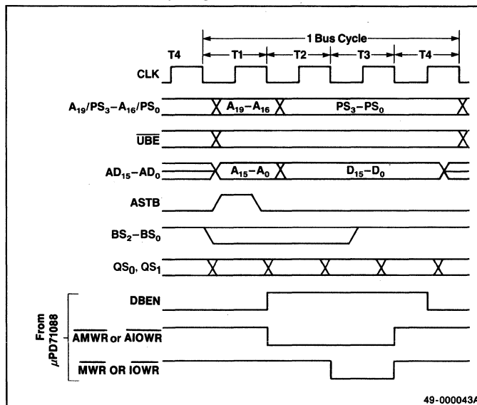
Figure 5-8. Write Timing of μPD70116 Memory and I/O (Large-Scale Systems)
