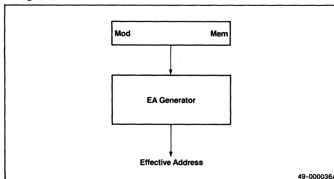
Figure 3-2. Effective Address Generator
