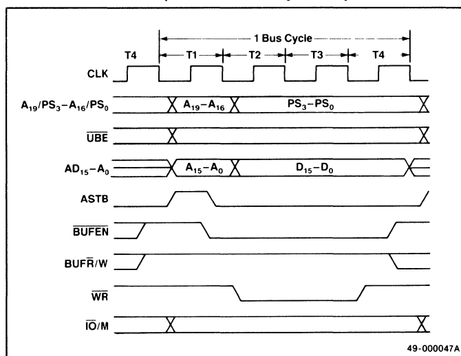
Figure 5-4. Write Timing of \mu PD70116 Memory and I/O (Small-Scale Systems)
