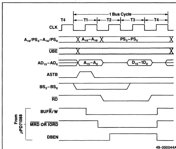
Figure 5-7. Read Timing of μPD70116 Memory and I/O (Large-Scale Systems)
