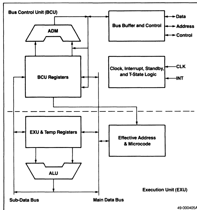
Figure 1-1. \mu PD70108/70116 Simplified Block Diagram
