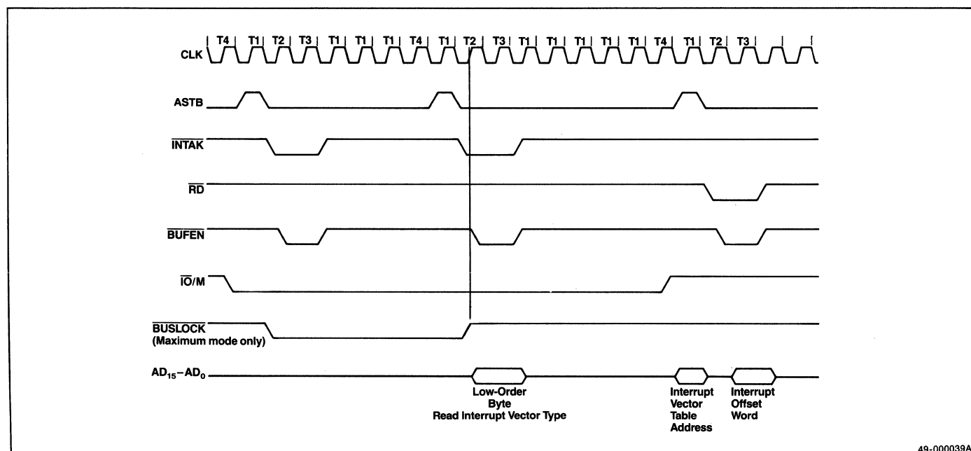
Figure 6-3. μPD70116 Interrupt Acknowledge Timing
