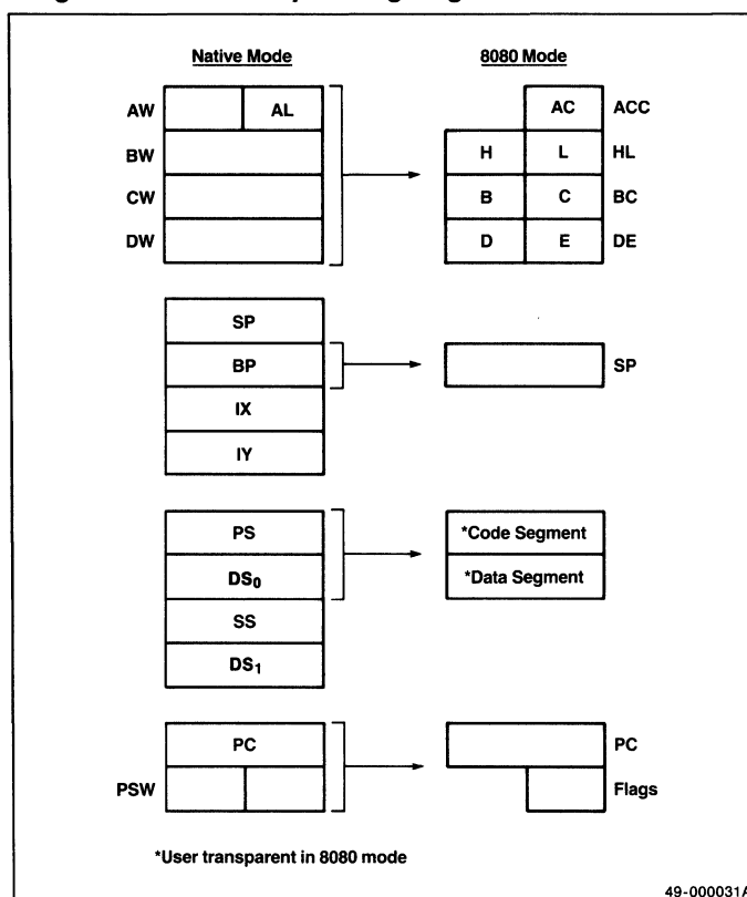
Figure 8.1. Corresponding Registers
