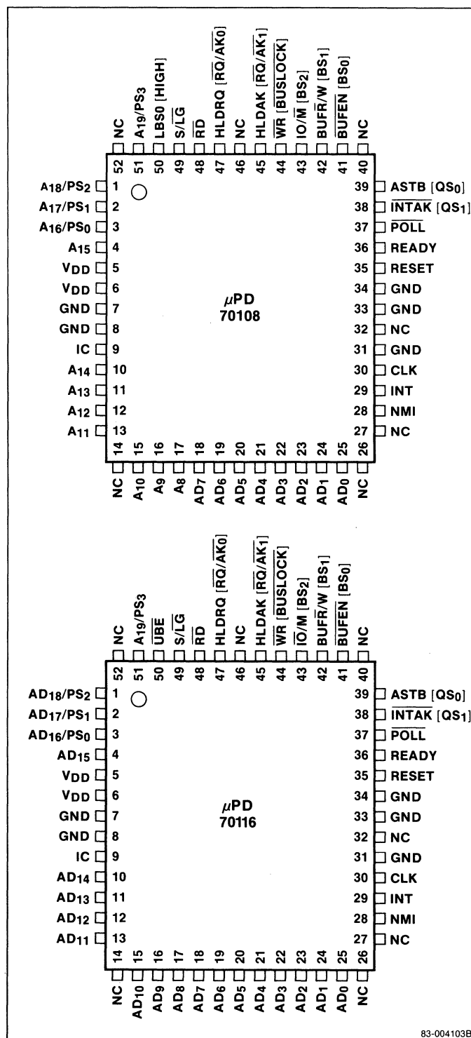
► Figure 1-4. Pin Configuration, 52-Pin Plastic Miniflat
