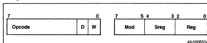
Figure 11-1. Bit Format
