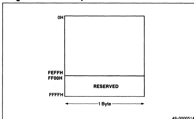
Figure 4-5. I/O Map
